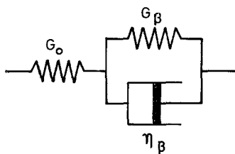
Figure 9 Simple three-element model used in Bauwens' treatment.
