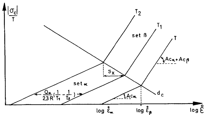
Figure 12 Graphical method of evaluating the constants of Equations 3 and 4 (schematic).
