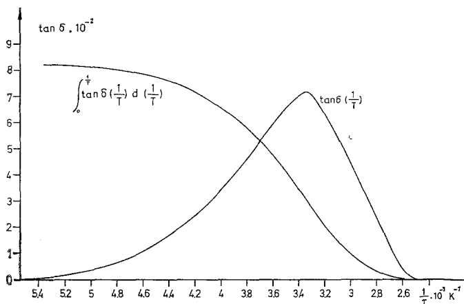
Figure 10 Contribution of peak p_{1b} to the \tan \delta (1/T) curve and integral of this contribution from 0 to 1/T .
