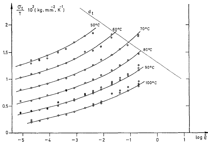
Figure 4 Ratio of tensile yield stress to temperature as a function of logarithm of strain-rate. The set of curves is generated by the shift of one curve along d_t , according to Equation 7. ( \dot{\epsilon} in \text{sec}^{-1} .)
