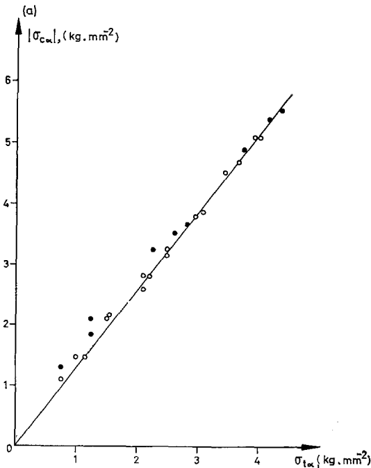
Figure 8 (a) Plot of the compression yield stress versus tensile yield stress, in the range of experimental conditions where only the \alpha process is involved in the deformation. The straight line drawn on the graph is calculated from Equation 12 using Table I. (b) Plot of the \beta contribution to the yield stress in compression versus the \beta contribution in tension (full circles: both quantities are measured; open circles: one quantity is measured while the other is extrapolated from the master curve). (c) Torsional yield stress as a function of pressure ( T = 25^\circ\text{C} , \dot{\gamma} = 4 \times 10^{-4} \text{ sec}^{-1} ). (Data of Ward et al [11]). The straight line drawn on the graph is calculated from Equations 19 and 20 using Table II.
